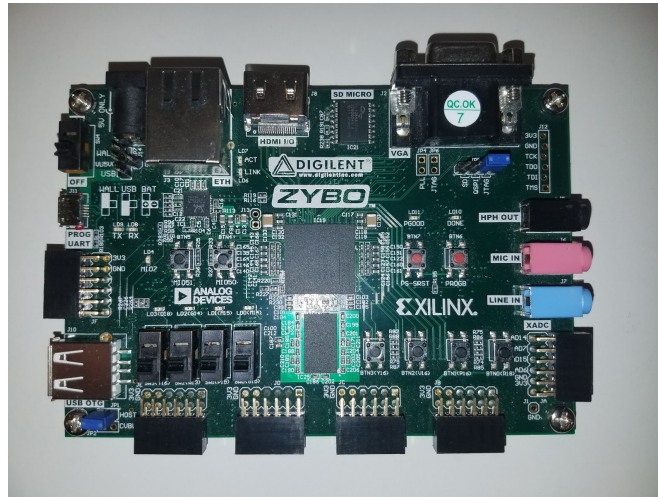
Figure 2: Zybo Board
